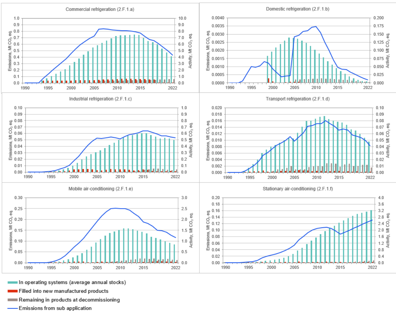
Figure 4.7-3 Total greenhouse gas emission and amounts of gas in operating systems, filled into new manufactured products and remaining in products at decommissioning of six subcategories of Refrigeration and air conditioning (Mt CO 2 eq.)
