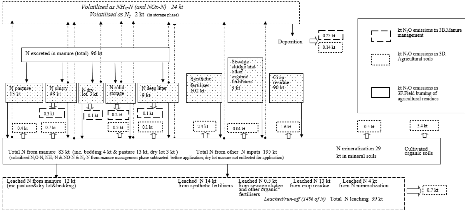
Figure 5.1-3 Nitrogen flows and nitrous oxide emissions in the Agriculture sector in 2022. Thin arrows denote N flows, of which dashed arrows show N volatilisation as ammonia, nitric oxide and dinitrogen. Bulk arrows denote N 2 O emissions. Nitrogen flows are in kt N year -1 and emissions (dotted line) in kt N 2 O year -1 . Figures are rounded, subtotals and totals calculated from unrounded values.
