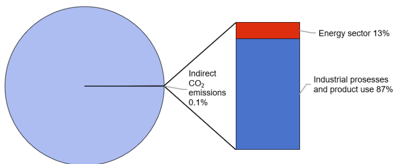
Figure 9.1-1 Indirect CO 2 emissions from the Energy sector and Industrial processes and product use compared with total emissions in 2022
