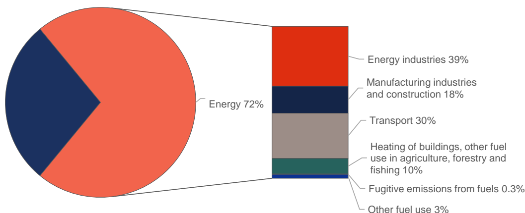
Figure 3.1-1 Emissions from the energy sector compared with total emissions in 2022. Due to independent rounding, the sums do not add up
