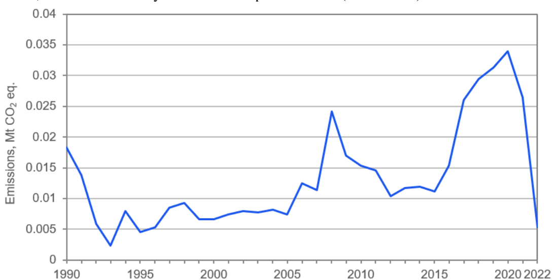
Figure 6.10-1 N 2 O emissions from forest fertilization (Mt CO 2 eq.)
