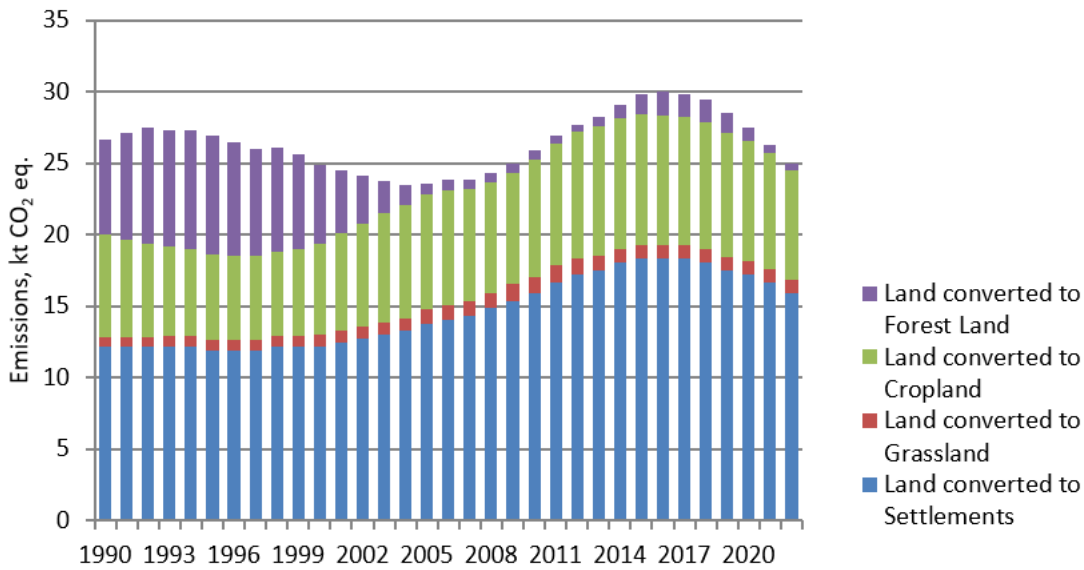
Figure 6.10-2 Direct and indirect N 2 O emissions from nitrogen mineralisation (kt CO 2 eq.)
