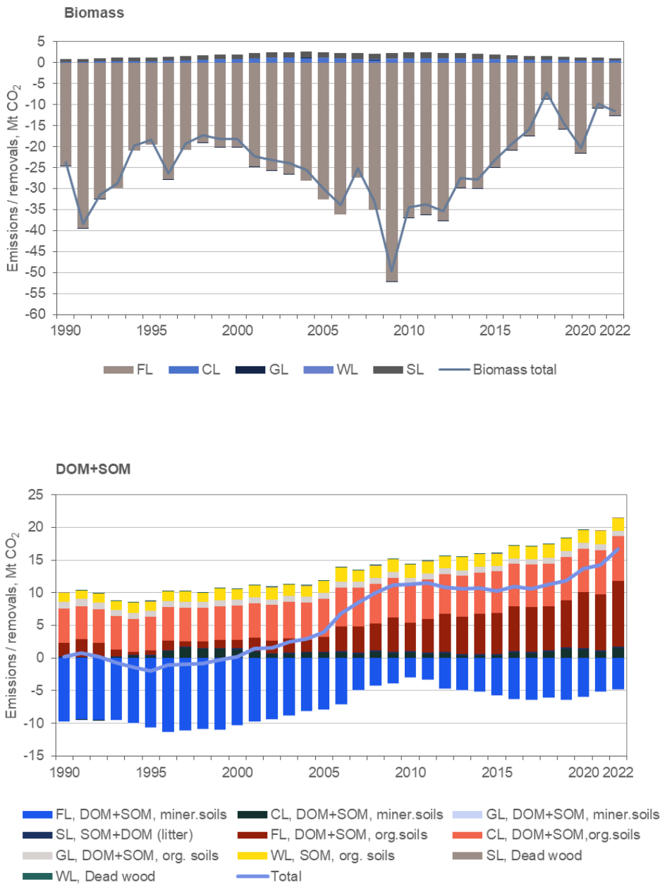
Figure 6.1-2 Emissions (positive sign) and removals (negative sign) from biomass (upper) and from soils (soil and dead organic matter) (lower) in different land use classes, Mt CO 2 . (FL = Forest Land, CL = Cropland, GL = Grassland, SL = Settlements, WL = Wetlands)
