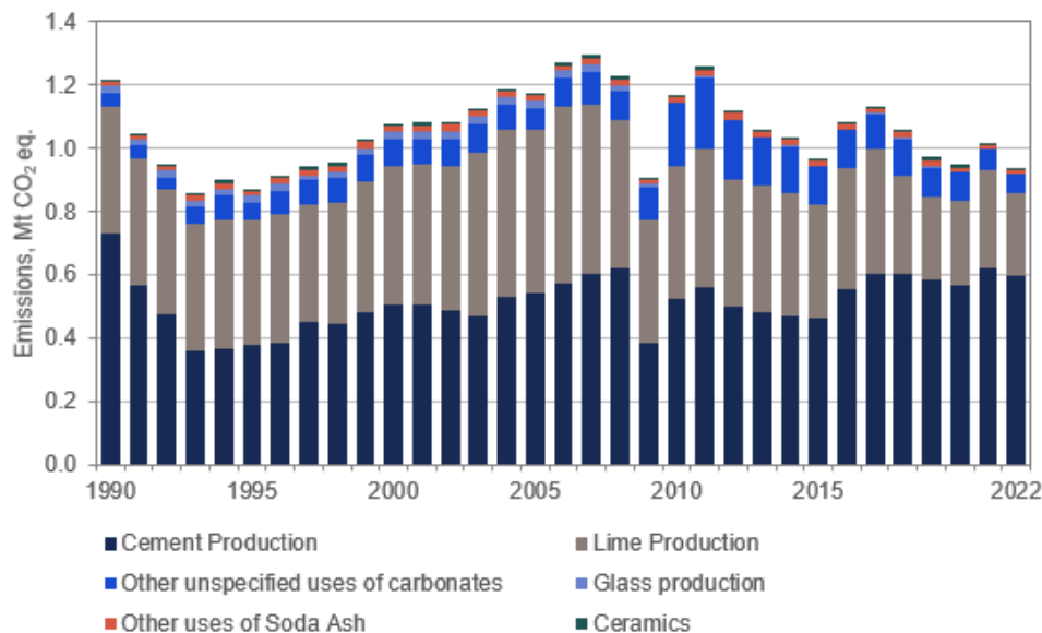
Figure 4.2-1 Greenhouse gas emission from Mineral industry (Mt CO 2 eq.)
