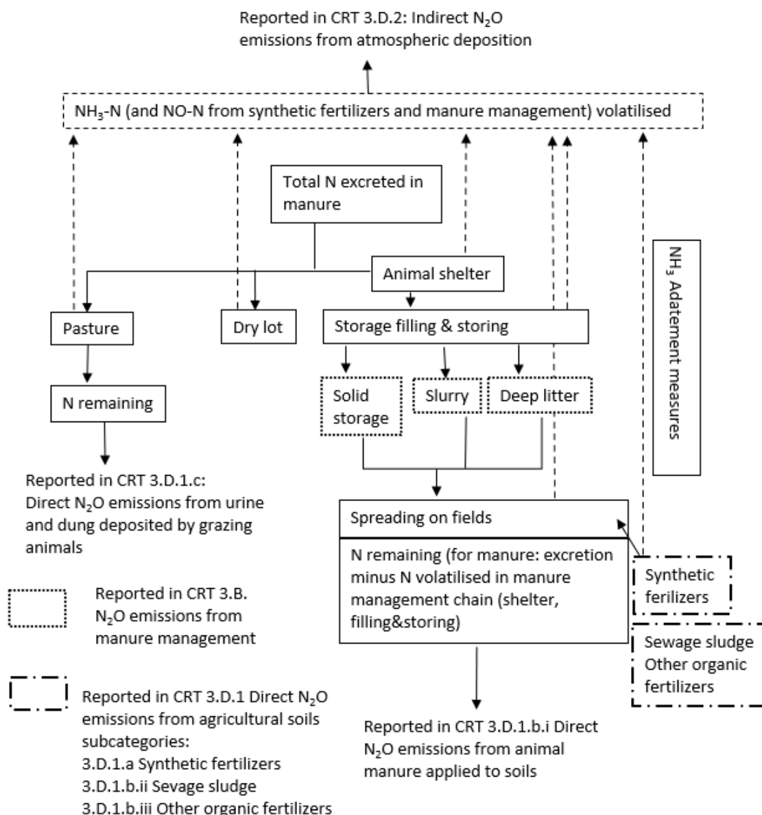
Figure 5.3-2 Distribution of manure N in the N flow model and reporting of direct and indirect N 2 O emissions from manure and inorganic fertilizers. Solid arrows describe N flows and broken arrows describe volatilised N as NH 3 -N (and NO x -N in case of inorganic fertilizers and manure storing). The magnitude of N 2 O emissions from each source is not presented here but in Figure 5.1-3. Dry lot manure remains in dry lot.
