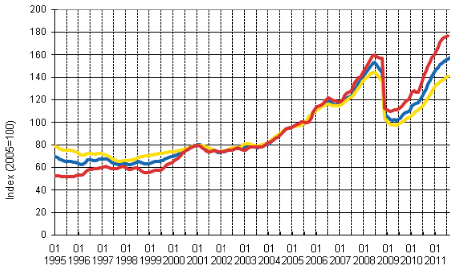
Appendix figure 3. Trend series on total turnover, domestic turnover and export turnover in the chemical industry 1/1995–10/2011
